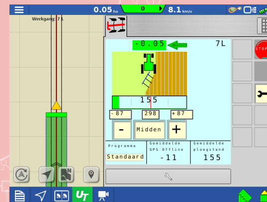
4. User Interface
